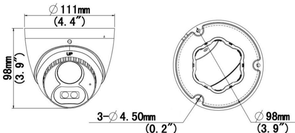
UAC-T124-AF28(40)LM
