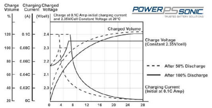
Typical characteristics for standby service type battery charge. Here, charging is continuous and the peak charge voltage must be lower.
