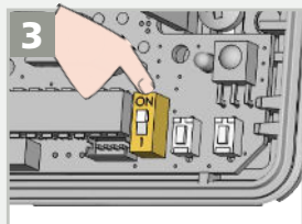
If mounting height is above 14' 6" (174"), activate BOOST function by DIP switch.
