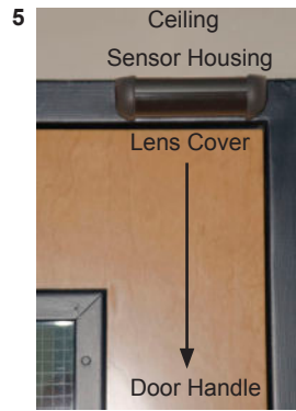
Install R2E-100 with Lens Cover Facing Down Toward Door Handle
