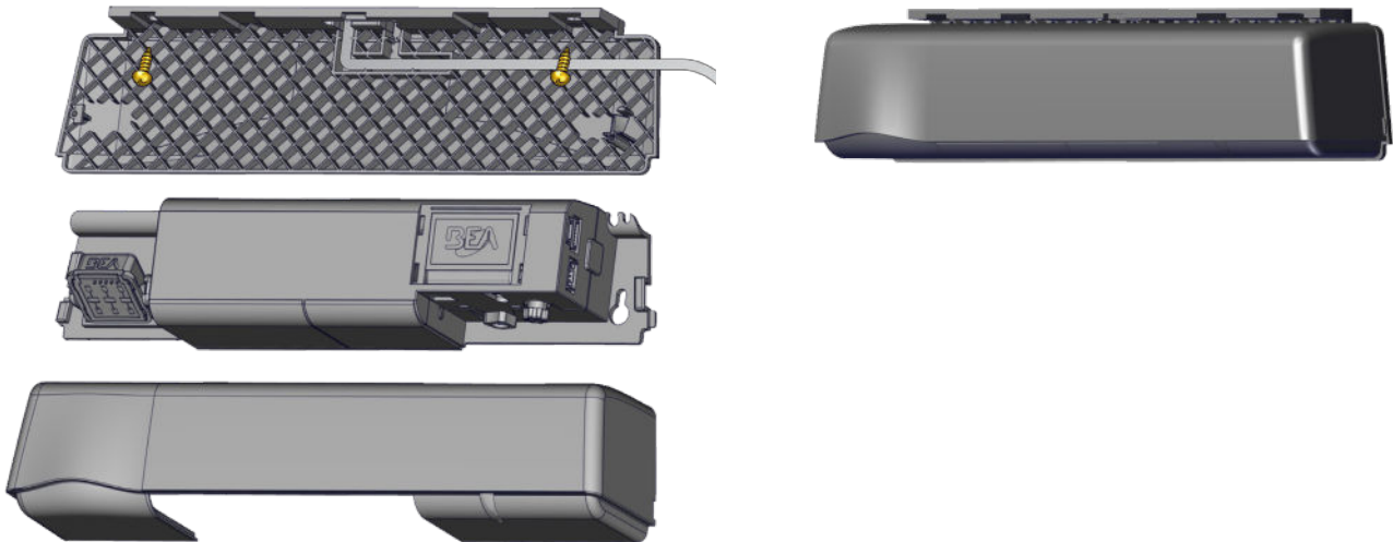
Exploded assembly with ULTIMO sensor
