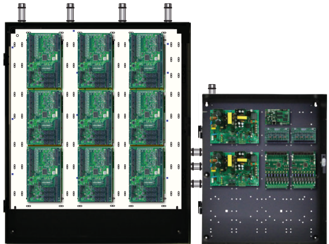
E8MH enclosure - 9 boards
