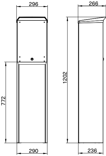
MS: View from front and from side
