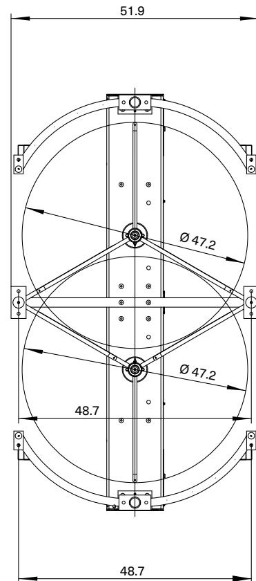
MPT 152/53/50 – 3-wing variants View from below
