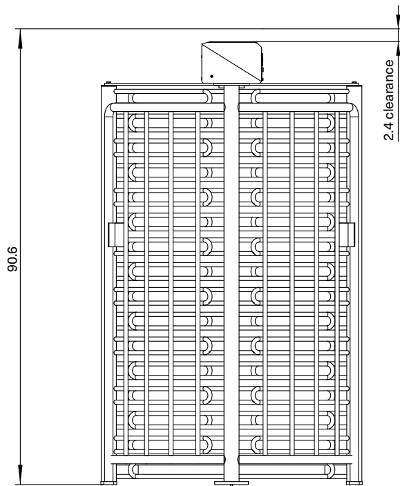
MPT 152/53/50 – 3-wing variants View from the side
